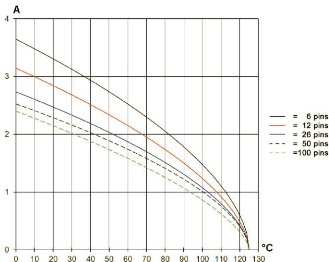
Derating curve @ I_{max} * 0.8 (IEC 60512-5-2)
