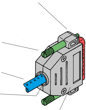
Cable with protective screen
